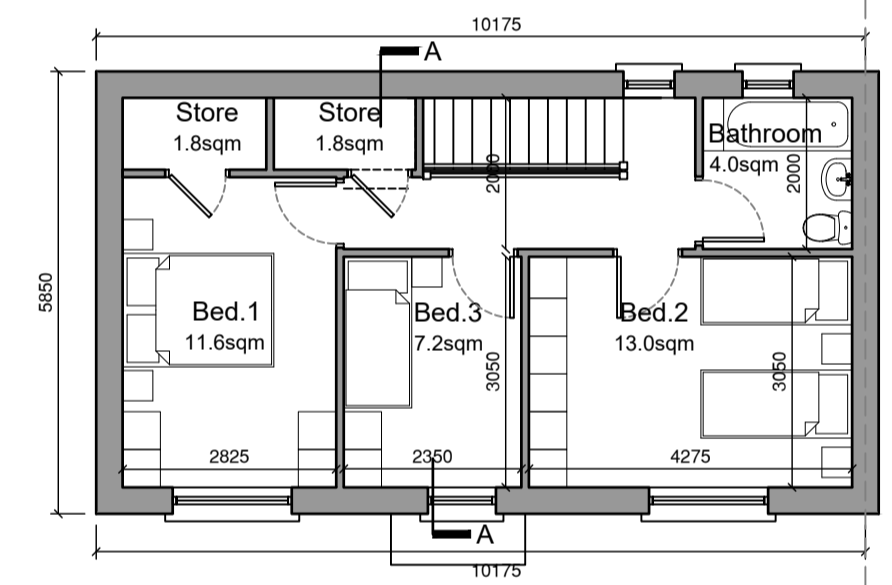
First Floor Plan Area:49.7sqm Total Floor Area 99.4sqm
